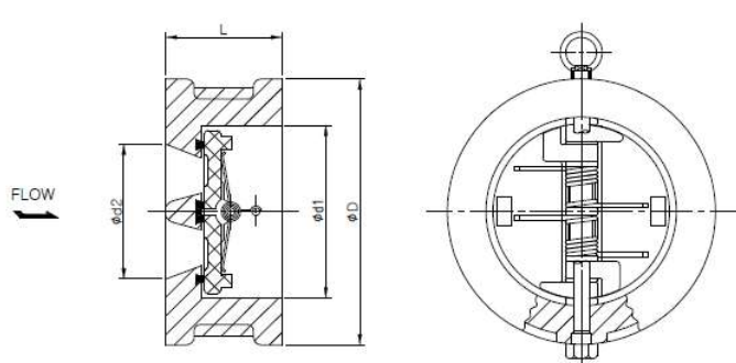
WAFER
